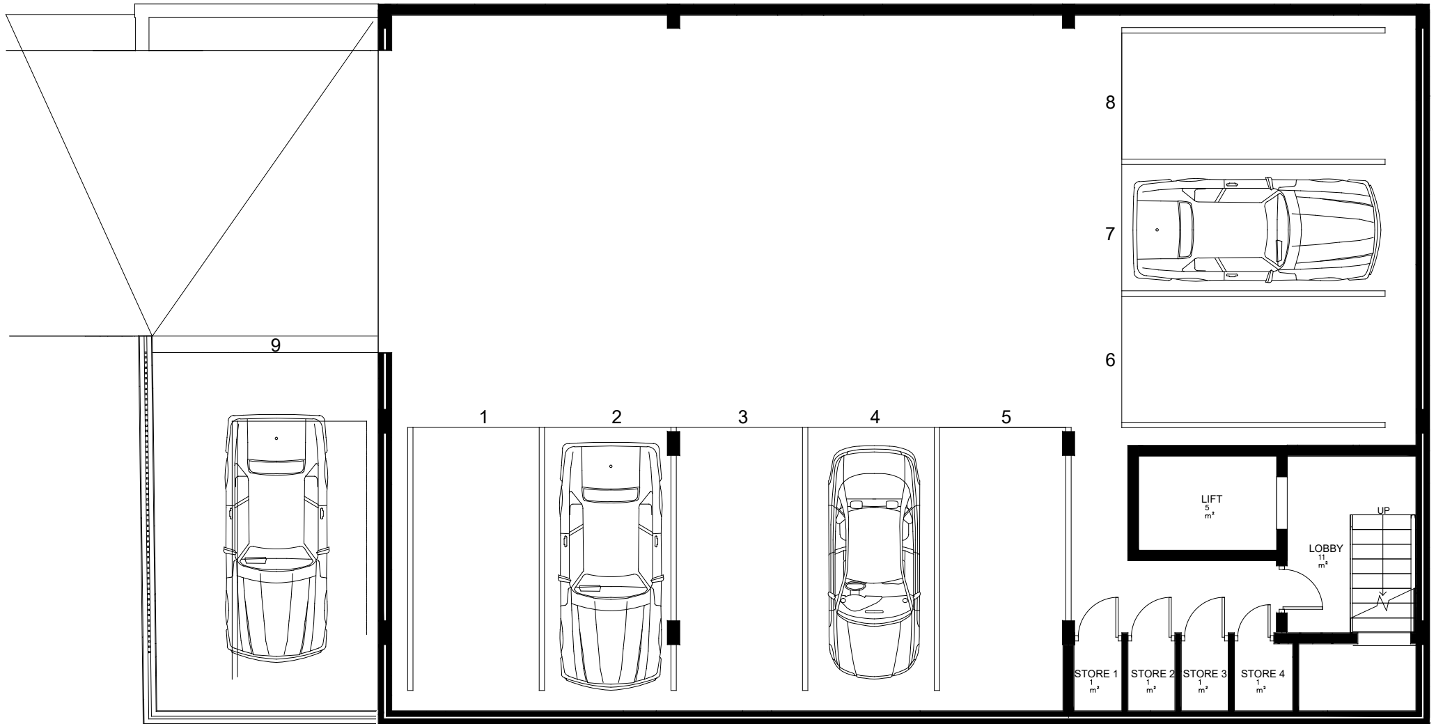
GROUND FLOOR PARKING scale 1 = 100
